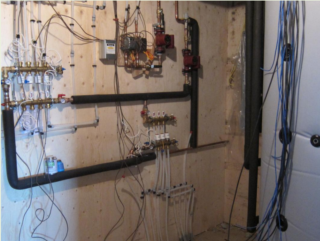
In-floor system and baseboard radiators are connected to the storage tank
